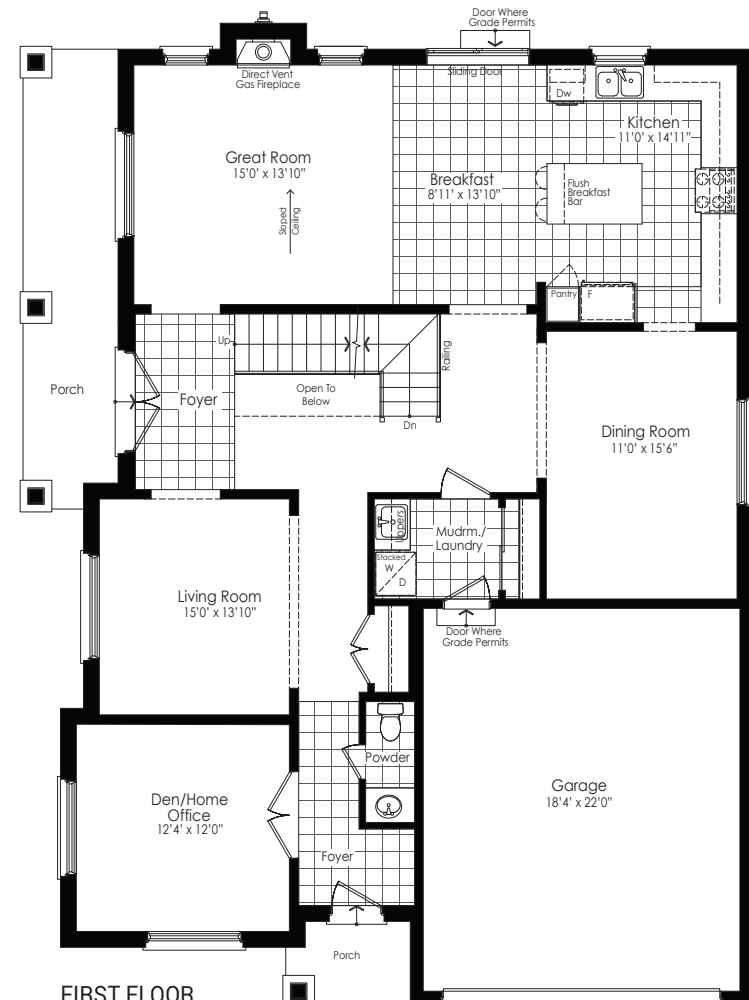
FIRST FLOOR ELEVATION B
